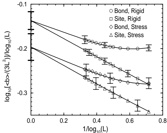
FIG. 12. The extrapolation of the fractal dimension and backbone dimension. The average number of bonds in a spanning cluster, \langle b \rangle , is determined at the rigidity threshold for both bond and site dilution. The spanning rigid and stressed regions lead to d_f and d_{BB} respectively. Only three typical error bars are shown on each data set for clarity.
