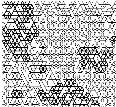
FIG. 3. The topology of a typical cut-out region from a bond-diluted generic network at p = 0.6603 . A particular realization would have local distortions (not shown) similar to Fig. 2. The heavy dark lines correspond to over-constrained regions. The open circles correspond to sites which are acting as pivots between two or more rigid bodies.
