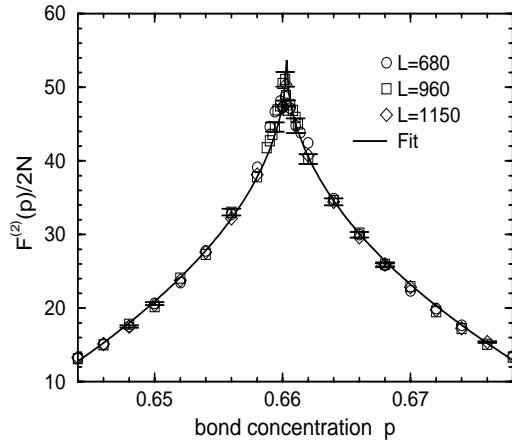
FIG. 7. The second derivative of the fraction of floppy modes for a bond diluted generic network as calculated from Monte Carlo sampling. The fitting results for the cusp yields p_{cen} = 0.6603 \pm 0.0003 and an exponent of 0.48 \pm 0.05 . Typical error bars are shown which reflect both the statistical errors in the Monte Carlo sampling and the ensemble averaging.
