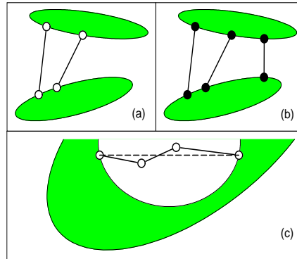
FIG. 1. The shaded regions represent 2d rigid bodies. The (closed, open) circles denote pivot-joints that are members of (one, more than one) rigid body. (a) A floppy piece of network with four distinct rigid clusters. (b) Three generic cross links between two rigid bodies make the whole structure rigid. If the bonds were parallel, the structure would not be rigid to shear[19]. (c) Three non-collinear connected rods connecting across a rigid body is generic and contains one internal floppy mode. If they were collinear (along the dotted line), then there would be two infinitesimal (not finite) floppy motions, and under a horizontal compression buckling would occur.
