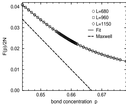
FIG. 5. Simulation results for the fraction of floppy modes, f = F/2N , for a bond diluted generic network compared to the Maxwell prediction. All error bars are smaller than the symbols. Note that the non-generic threshold[12] is at 0.641.
