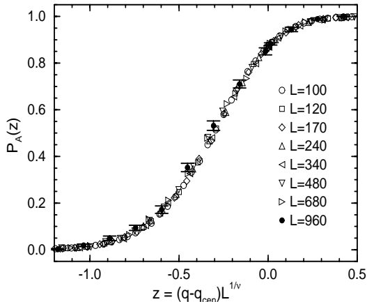
FIG. 11. The probability for a site-diluted system with periodic boundaries to percolate rigidity, P_A(q, L) , is plotted against the scaled axis z = (q - q_{cen})L^{1/\nu} with q_{cen} = 0.69755 and \nu = 1.21 . We note that when using the same value of the threshold, the best data collapse is obtained with a \nu of 1.25, and that a good data collapse can be found with \nu in the range between 1.22 and 1.28. Error bars are shown for system size L = 960 . Generally the error bars are the biggest when P_A \approx 0.5 for any size L , and increase as L increases because fewer realizations are generated. Also see Fig. 8 which has the same trend.
