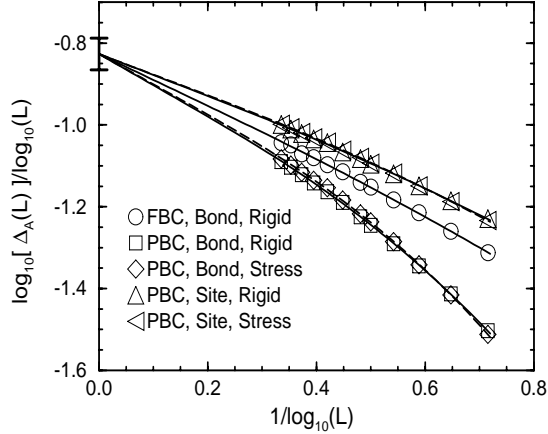
FIG. 9. An extrapolation for the exponent \nu (as 1/\log_{10}(L) \rightarrow 0 ) given by the inverse of the negative of the y-intercept. An accurate estimate is made with five data sets simultaneously fitted to Eq. (10). Error bars are approximately the size of the symbols. The solid (dashed) lines denote the extrapolated best fit (with \nu = 1.21 and c = 0.59 ) for \Delta_A(L) corresponding to spanning rigid (stressed) regions. The error bar at the extrapolated best value takes into account other comparatively good extrapolations. Note that the fluctuations in finding a network to percolate rigidity and stress are nearly the same.
