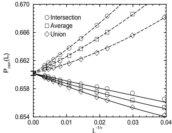
FIG. 10. The extrapolation of the rigidity threshold for bond dilution as L^{-1/\nu} \rightarrow 0 . The different symbols represent data from three separate calculations using the distributions P_I , P_A and P_U defined in the text. The symbol sizes reflect typical error bars. The dashed and solid lines show the best-fit curves to the data with free and periodic boundary conditions respectively. Here we have fixed \nu = 1.21 and show the results from simultaneously fitting all six data sets to the form given by Eq. (11) where we find p_{cen} = 0.6602 and c = 0.733 . The error bar at the extrapolated value takes into account other comparatively good extrapolations.
