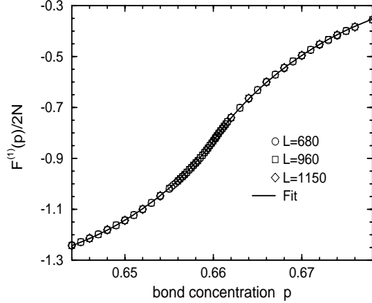
FIG. 6. The first derivative of the fraction of floppy modes for a bond diluted generic network as calculated exactly from Eq. (5). All error bars are smaller than the symbols.
