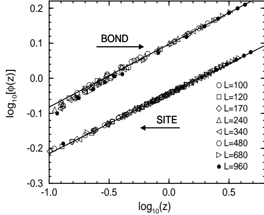
FIG. 14. Taking the data in Fig. 13, we plot the \log_{10} of the scaling function, \phi(z) , versus the \log_{10} of the scaling variable, z , (for z > 0 ) in order to estimate the \beta exponent from the slope of an expected straight line. We show a least squares fit (fitting over the top \approx 50\% of the data points shown) that is extended through all the data points for the bond and site dilution data separately. The slopes are found to be 0.179 and 0.171 for the bond and site data respectively.
