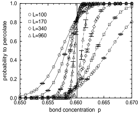
FIG. 8. The probability for a bond-diluted generic network to percolate rigidity, P_A(p, L) , is plotted for periodic (free) boundary conditions for various system sizes with solid (dashed) line segments drawn between data points. Only four different sizes and several typical error bars are shown for clarity. The vertical solid line indicates our extrapolated threshold.
