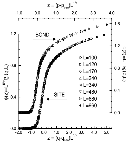
FIG. 13. The probability for a bond to be on the incipient infinite rigid cluster, P_\infty , is scaled by a factor of L^{\beta/\nu} for linear system sizes ranging from L = 100 to L = 960 . We plot the scaled data, representing the scaling function \phi(z) , for both a bond and site diluted system with periodic boundaries using the top-right and bottom-left axes respectively. In this plot, we used \nu = 1.21 , \beta = 0.175 , q_{cen} = 0.69755 and p_{cen} = 0.66020 .
