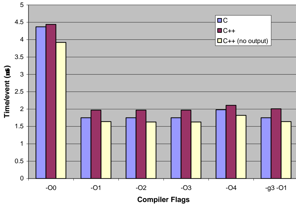
Level 2 C/C++ Framework Timings
