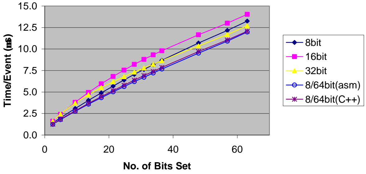
Event Time vs. Number of Bits for Different Search Block Sizes
