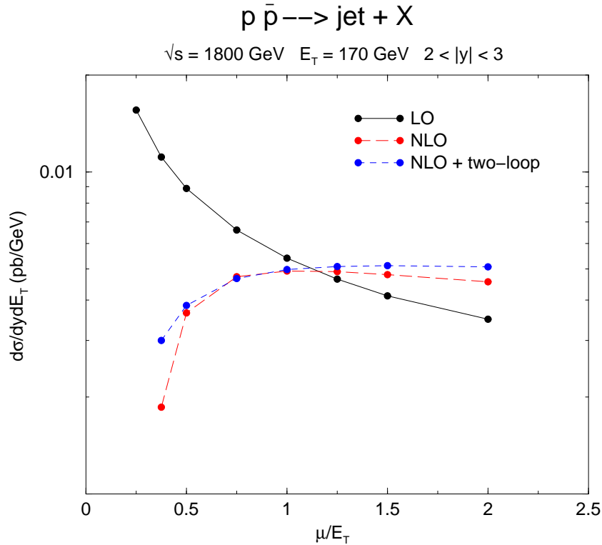
Figure 22: Same as Fig.17 with the addition of the estimated two-loop contribution expected from threshold resummation.
