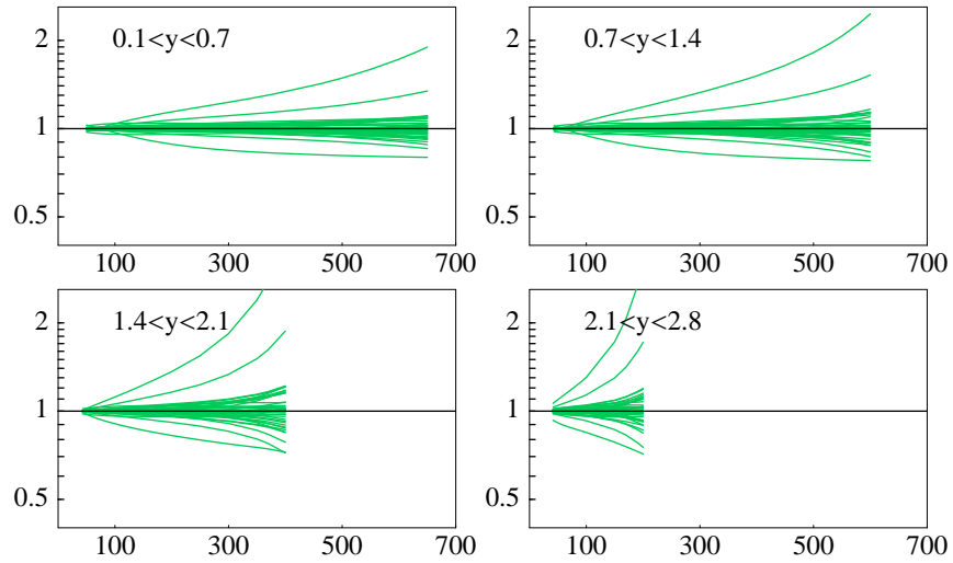
Figure 28: Uncertainty range of the Run 2 cross section for the CDF rapidity bins. The curves show the ratios of the 40 eigenvector basis sets compared to the central (CTEQ6.1M) prediction (ordinate) versus p_T in GeV (abscissa). The dotted curves are the effect of a compositeness scale of 2.4 TeV.
