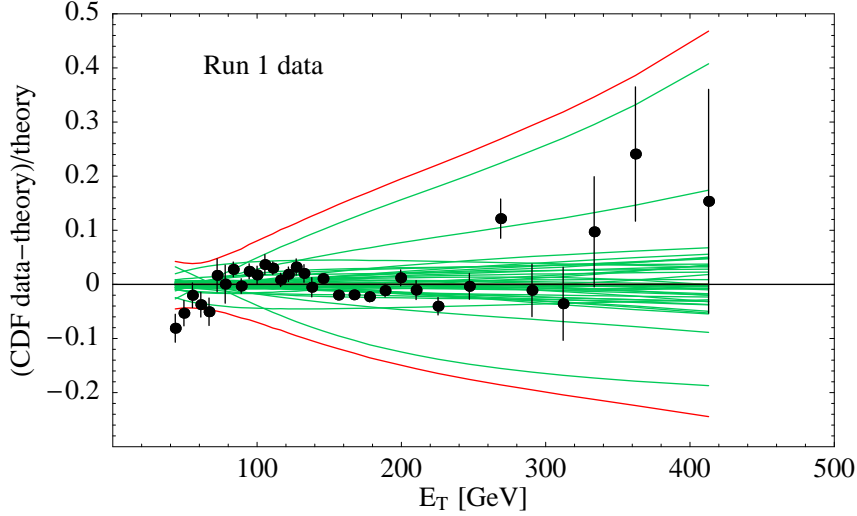
Figure 12: The overall PDF uncertainty of the inclusive jet cross section is plotted as the two red curves. The points are CDF data; the error bars are statistical only and the systematic shifts have not been subtracted.
