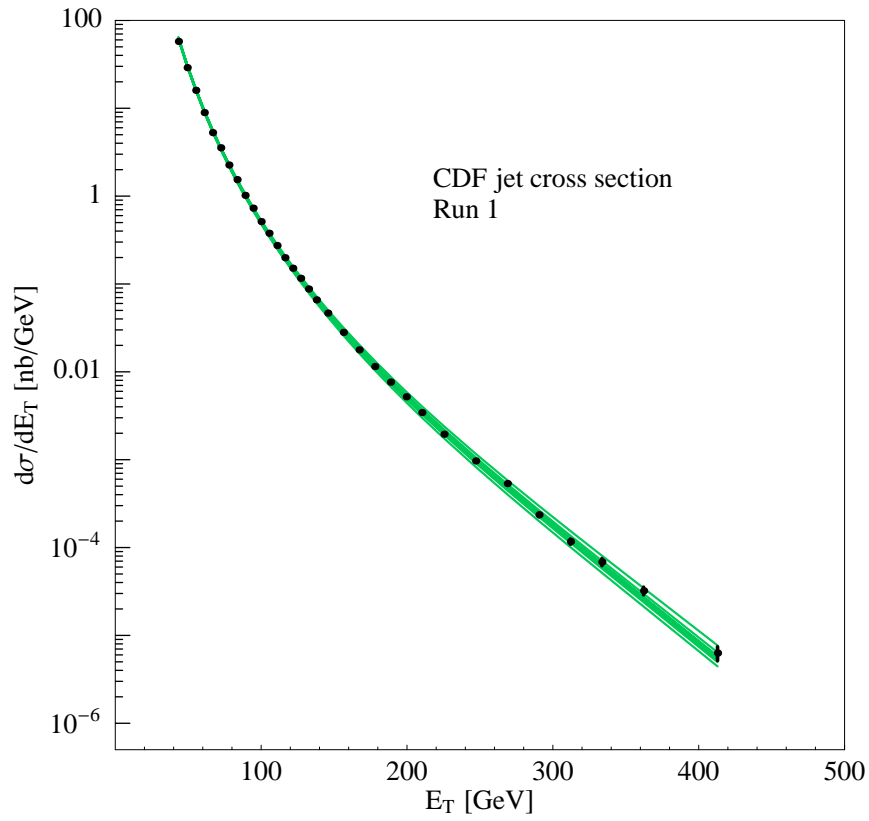
Figure 9: Calculations of d\sigma/dE_T for the 40 eigenvector sets.
