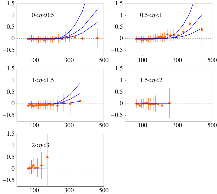
Figure 23: Comparison of three models in which a hypothetical contact interaction contributes to jet production. The ordinate is the fractional difference between the model and the standard theory; the abscissa is the jet E_T in GeV. The contact interaction has \Lambda = 1.6, 2.0, and 2.4 TeV for the three curves. In all cases the PDF's are the standard CTEQ6.1M. The DØ data are superimposed for comparison.
