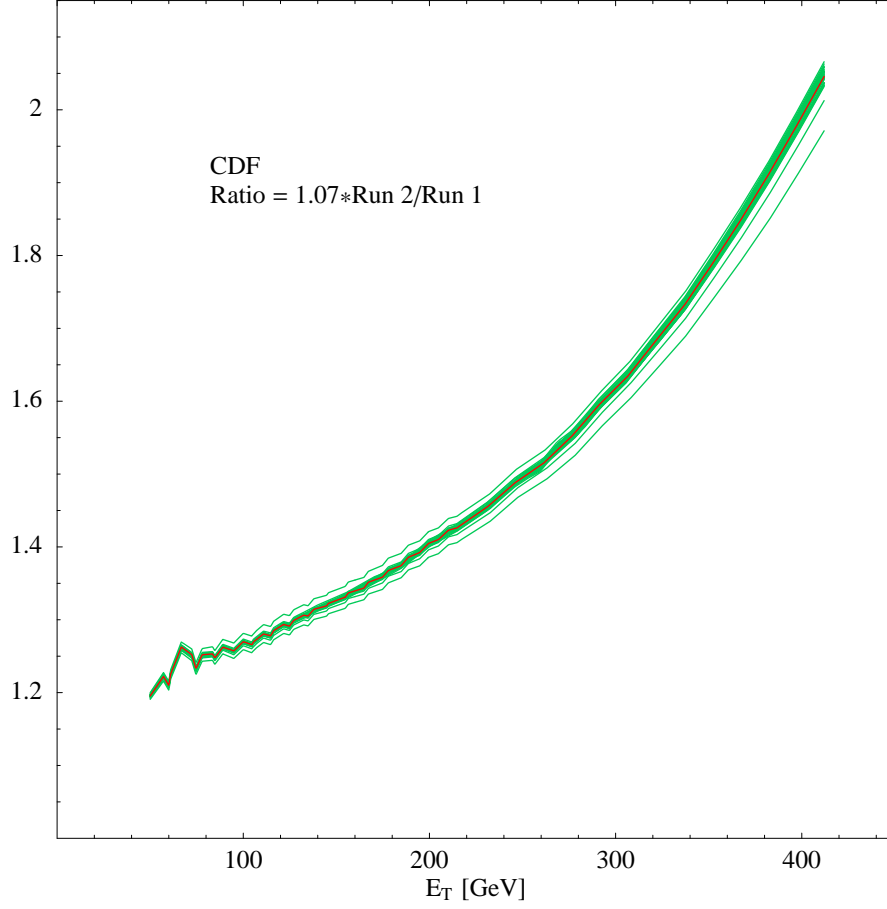
Figure 29: The ratio of the Run 2 to Run 1b cross sections for the central rapidity range ( 0.1 < |\eta| < 0.7 ). The Run 2 cross section has been multiplied by 1.07 to take into account the difference in the jet definitions for the Run 2 and Run 1b analyses. (The small fluctuations are due to the Monte Carlo errors in the calculations of the K-factors (NLO/LO) at each energy.)
