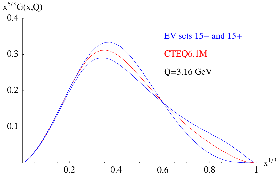
Figure 13: Eigenvector 15. Comparison between the gluon distributions for the + and – displacements along eigenvector 15 and the standard set CTEQ6.1M.
