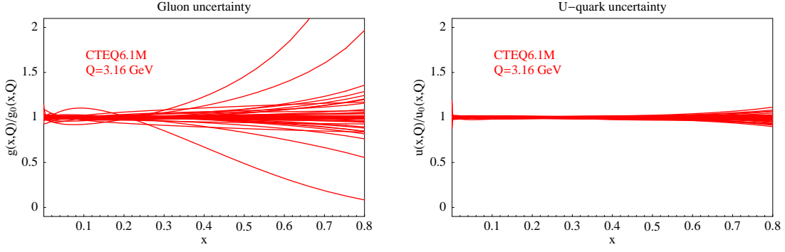
Figure 6: PDF uncertainties. The curves are the ratios of the 40 eigenvector basis sets to the standard set (CTEQ6.1M). The largest variations of the gluon function are the + and – displacements along eigenvector 15.
