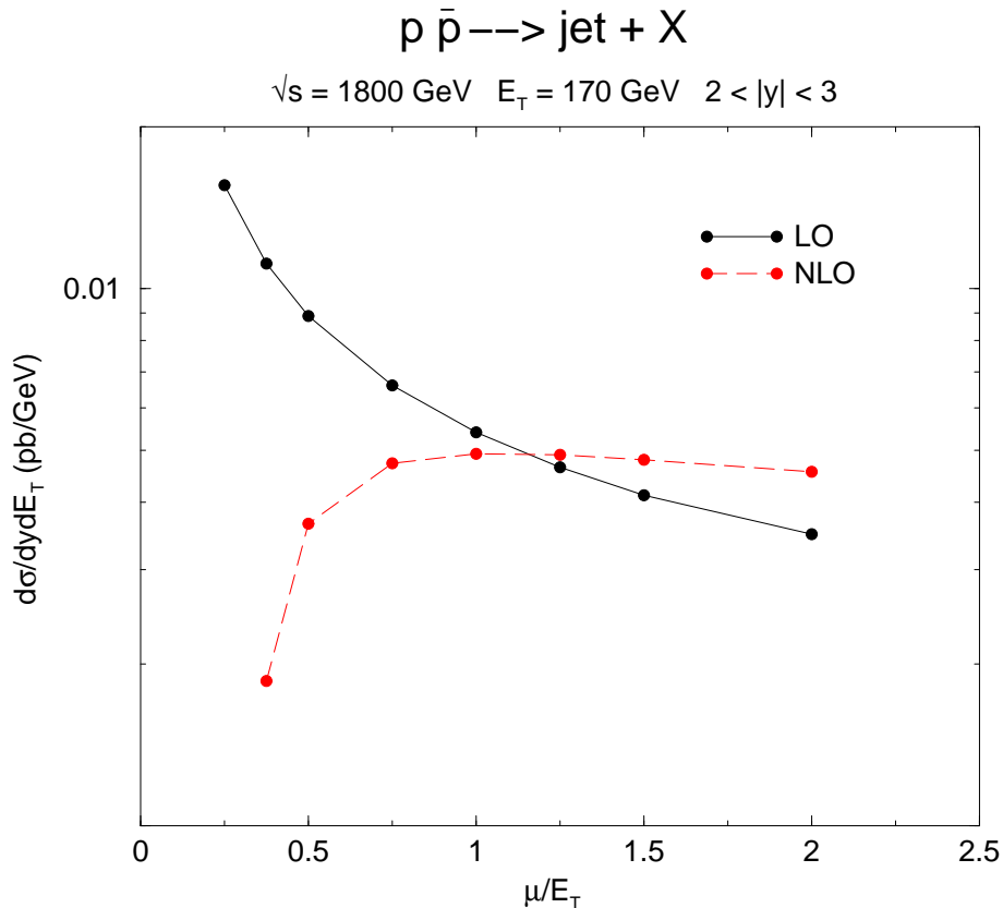
Figure 17: Comparison of the scale dependence of the jet cross section at E_T=170 GeV/c for the leading- and next-to-leading-logarithm calculations
