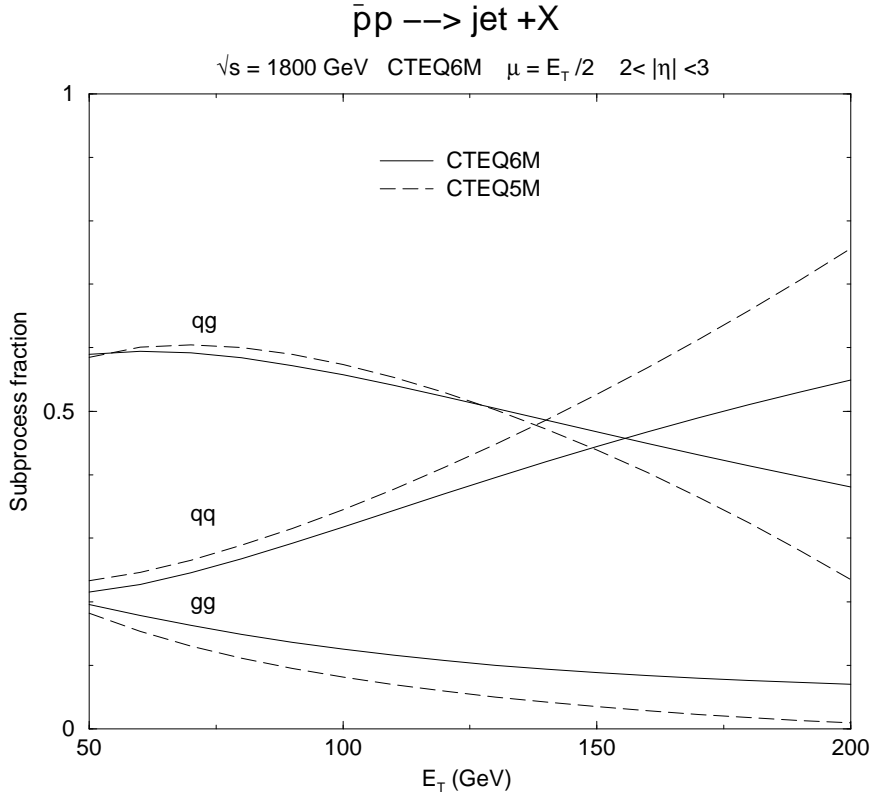
Figure 4: The subprocess contributions to jet production in the forward rapidity region.
