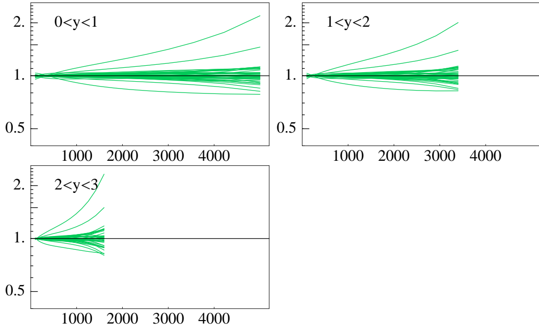
Figure 31: The uncertainty range of the inclusive jet cross section at the LHC. The curves are graphs of the ratios of the cross sections for the 40 eigenvector basis sets compared to the central (CTEQ6.1M) prediction (ordinate) versus p_T in GeV (ordinate).
