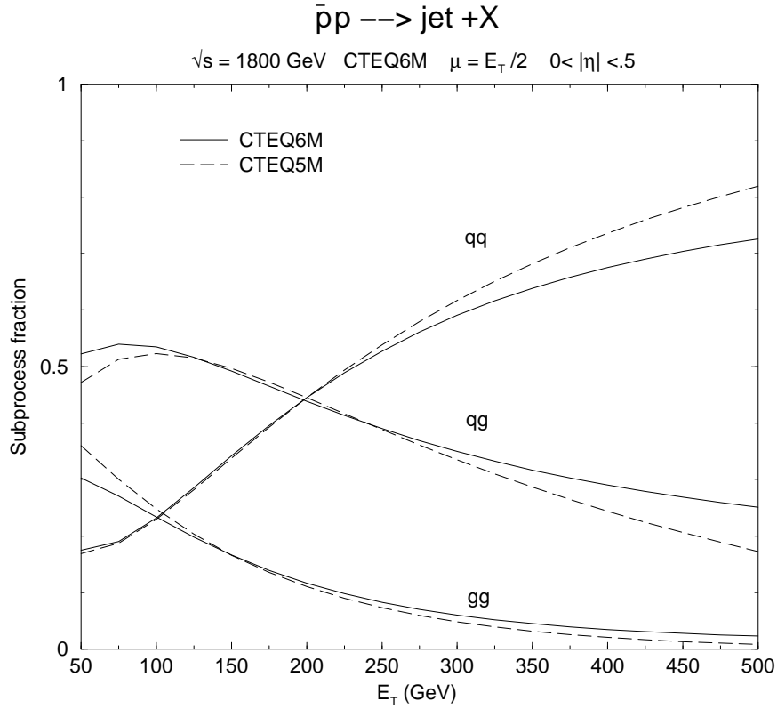
Figure 3: The subprocess contributions to central jet production.
