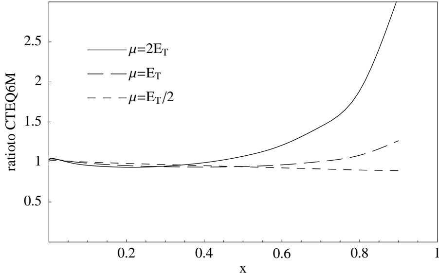
Figure 18: Comparison of fitted gluon distributions for fits made with different scale choices for the jet cross section. Comparison to Fig.6 shows that this theoretical error is smaller than the uncertainty due to experimental errors.
