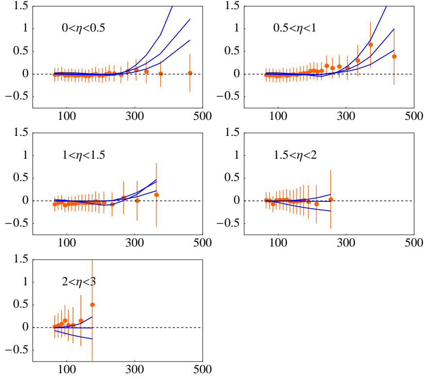
Figure 24: Comparison of three models in which a hypothetical contact interaction contributes to jet production, with refitting of the PDF's. The curves have the same meaning as in Fig. 23. The PDF's for the three models have been refit to the global data set to give the best fit including the contact interaction in jet production.
