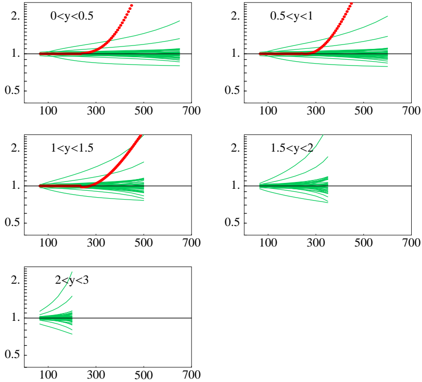
Figure 26: Uncertainty range of the Run 2 cross section for the DØ rapidity bins. The curves show the ratios of the 40 eigenvector basis sets to the central (CTEQ6.1M) prediction (ordinate) versus p_T in GeV (abscissa). The red curve is the effect of a compositeness scale of 2.4 TeV.
