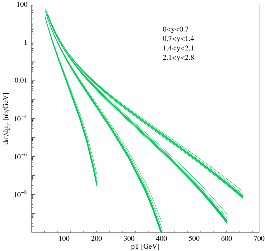
Figure 27: Run 2 cross section for the CDF rapidity bins.
