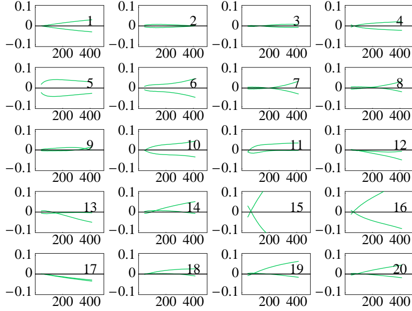
Figure 11: The cross sections for + and - displacements along the 20 eigenvectors, plotted as fractional differences compared to CTEQ6.1M.
