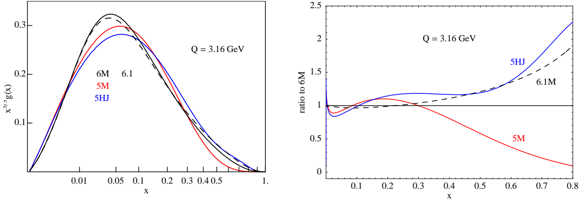
Figure 2: Left: The CTEQ5M, CTEQ5HJ, and CTEQ6M gluon distributions at Q^2 = 10 \text{ GeV}^2 . Right: The ratios of CTEQ5M and CTEQ5HJ gluon distribution to that of CTEQ6M. The dashed curves show the CTEQ6.1M gluon distribution.
