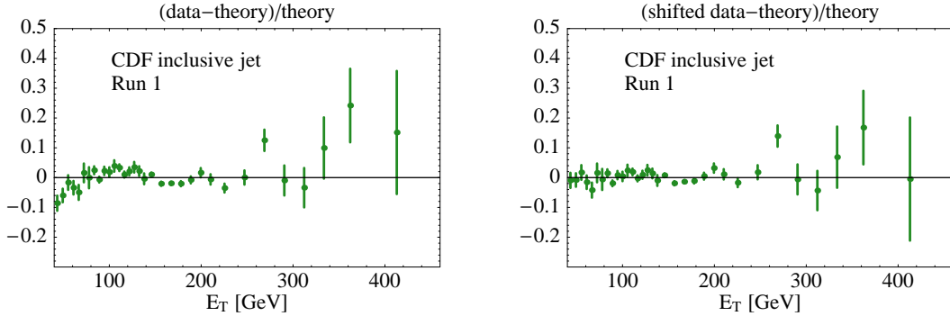
Figure 8: The left panel shows (D_i - T_i)/T_i , the fractional difference between data and theory. The right panel shows (\overline{D}_i - T_i)/T_i where \overline{D}_i is the data with systematic shifts subtracted. The error bars are the statistical errors only.
