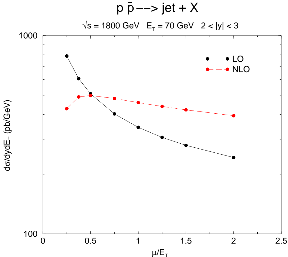
Figure 16: Comparison of the scale dependence of the jet cross section at E_T=70 \text{ GeV}/c for the leading- and next-to-leading-logarithm calculations
