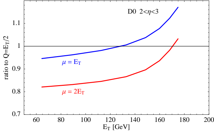
Figure 20: Scale dependence of the jet cross section prediction for 2 < y < 3 .
