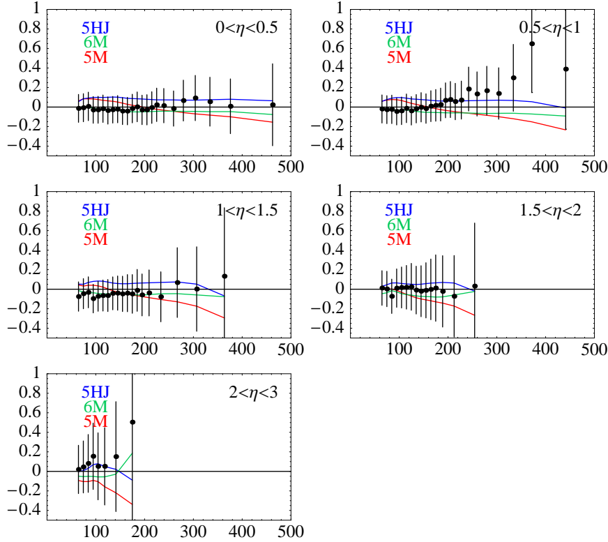
Figure 1: The D\bar{0} inclusive jet cross section versus E_T for five rapidity bins compared to NLO predictions using the CTEQ6.1M PDF's. The abscissa is E_T in GeV. The ordinate is (\text{data} - \text{theory})/\text{theory} . The curves show the CTEQ5M, CTEQ5HJ, and CTEQ6M predictions, as fractional differences compared to CTEQ6.1M. The error bars are the statistical and systematic errors combined in quadrature.
