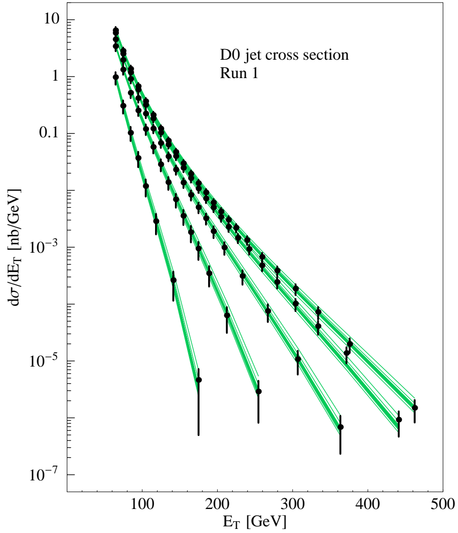
Figure 14: The inclusive jet cross section as a function of E_T for the five rapidity bins of the Run 1b D0 measurements. Predictions of all 40 eigenvector basis sets are superimposed. The points are the D0 data, and the error bars are the statistical and systematic errors combined in quadrature.
