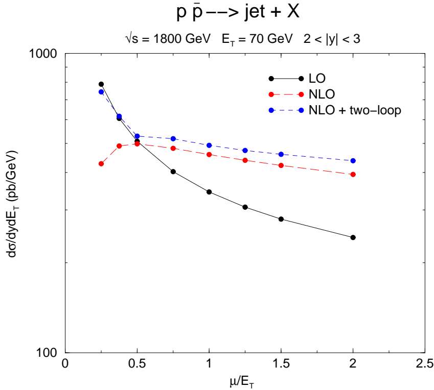
Figure 21: Same as Fig. 16 with the addition of the estimated two-loop contribution expected from threshold resummation.
