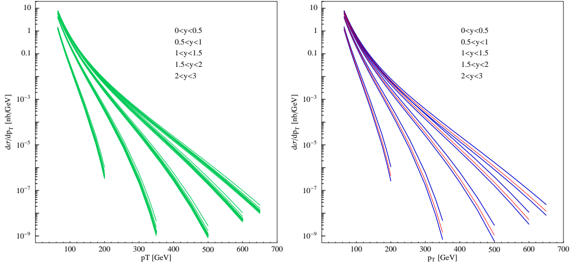
Figure 25: Run 2 cross section for the D\emptyset rapidity bins. Left: The 40 eigenvector basis sets. Right: The central prediction and overall uncertainty band.
