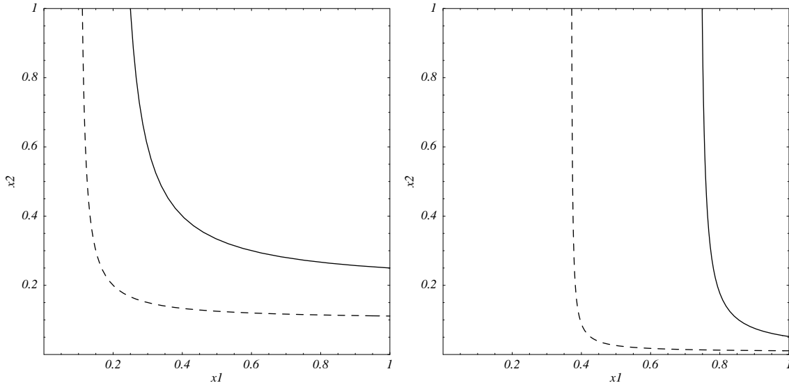
Figure 5: Left: Parton momentum fractions x_1 and x_2 for y_j = 0 ; the solid and dashed curves are for E_T = 400 and 200 GeV, respectively. Right: Parton momentum fractions x_1 and x_2 for y_j = 2 ; the solid and dashed curves are for E_T = 200 and 100 GeV, respectively.
