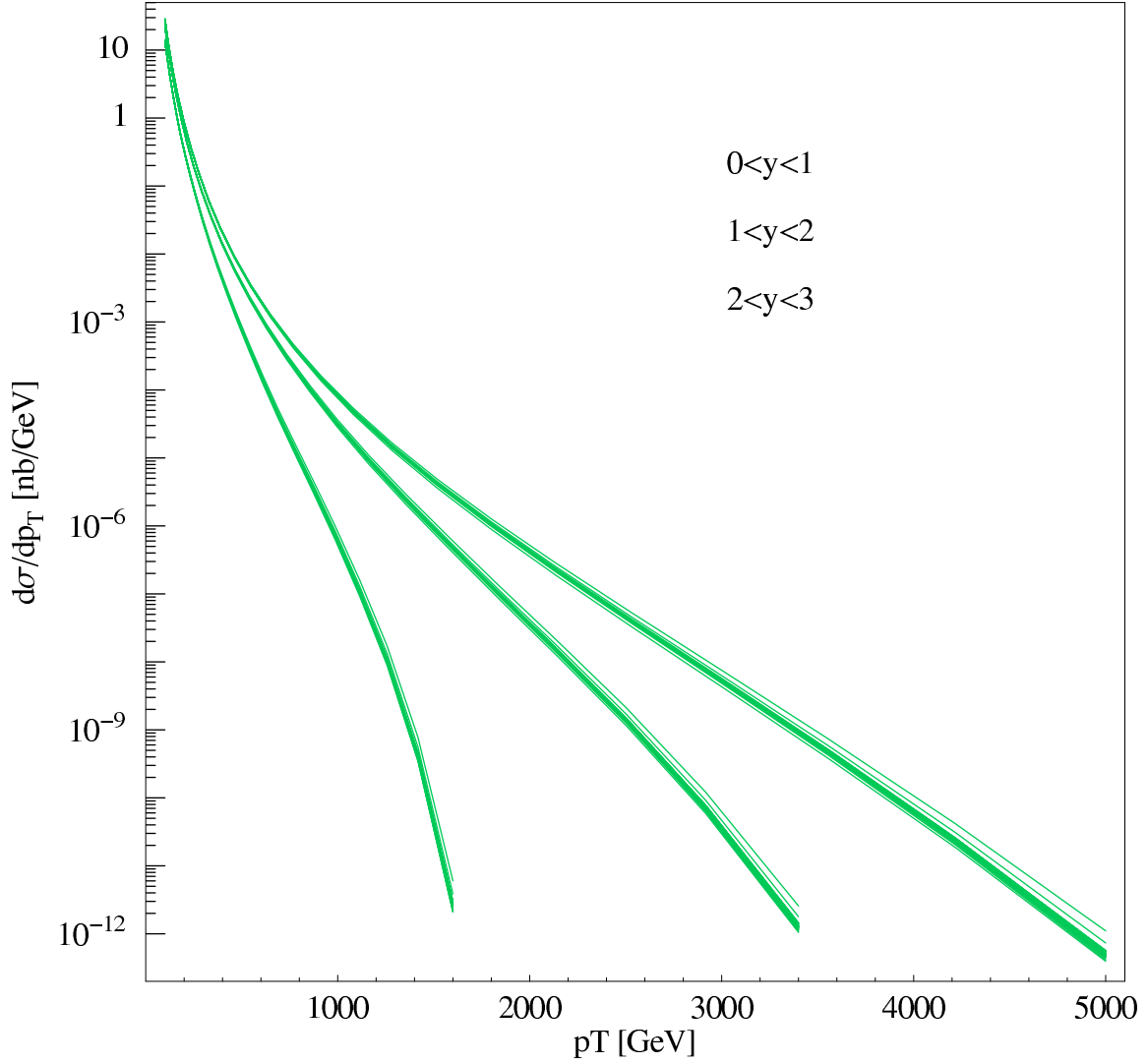
FIG. 30: The inclusive jet cross section as a function of p_T for three rapidity bins at the LHC. The three rapidity ranges are (0, 1), (1, 2) and (2, 3). Predictions of all 40 eigenvector basis sets are superimposed.
