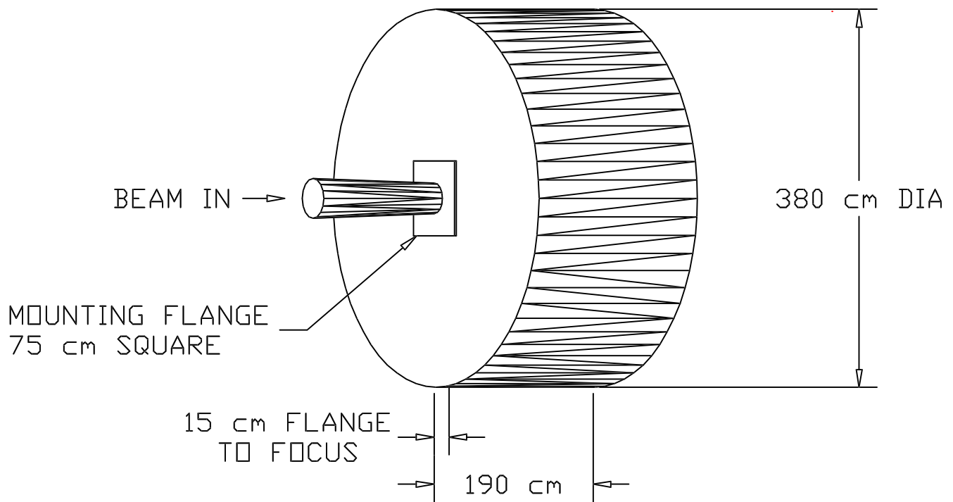
SOAR INSTRUMENT CLUSTER: AVAILABLE VOLUME FOR STRAIGHT- THROUGH INSTRUMENT POSITION
