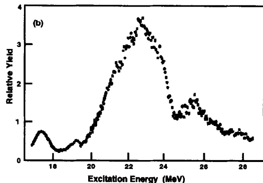
Fig. 3. Comparison of the giant dipole plasmon resonances observed in (a) the C_{60} molecule via photoionization with synchrotron radiation [9], and (b) the ^{12}\text{C} nucleus via the ^{11}\text{B}(p, \gamma)^{12}\text{C} reaction [11].
