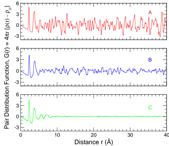
Figure 2. The calculated PDF for a 100,000 atom model. 12 of amorphous silicon with a mean Si - Si nearest neighbour distance of 2.4\text{\AA} and with a thermal width that approaches \sigma = 0.1\text{\AA} at larger distances. The panels A, B, C are for a single atom at the origin, averaged over 10 atoms at the origin, and averaged over 20000 atoms at the origin respectively.
