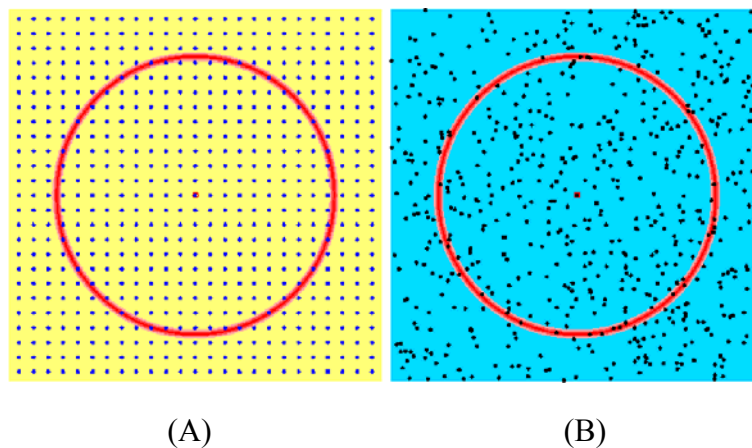
Figure 1. (A) a regular grid of points is enclosed by a circle, while in (B) there is a set of random points. To calculate the pair distribution function (PDF) one point is chosen as the origin of a circle of radius r . Only those sites inside the red annulus of width \sigma contribute to the value of PDF at a distance r .
